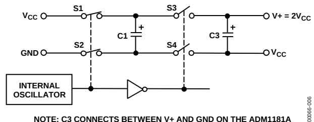
Figure 6. Charge-Pump Voltage Doubler
