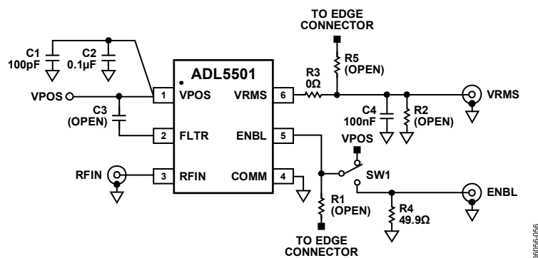
Figure 56. Evaluation Board Schematic
