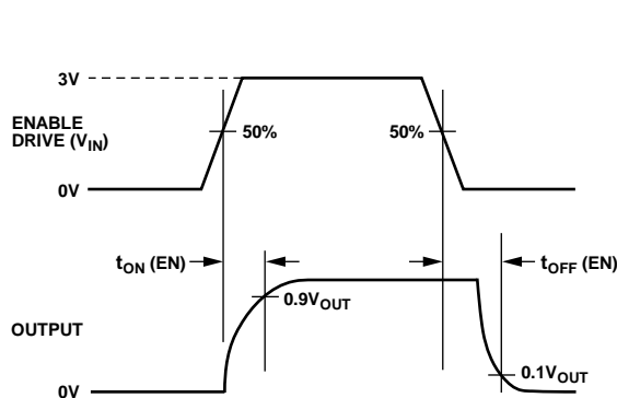
Figure 36. Enable Delay, t_{\text{ON}}(\text{EN}) , t_{\text{OFF}}(\text{EN})
