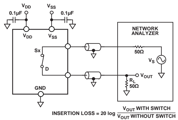
Figure 41. Bandwidth
