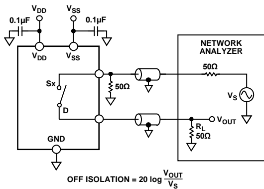
Figure 39. Off Isolation
