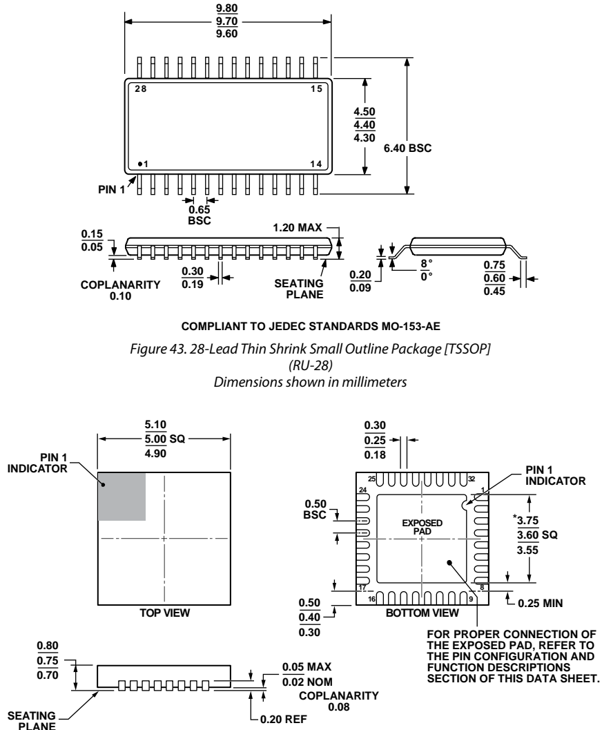
Figure 44. 32-Lead Lead Frame Chip Scale Package [LFCSP_WQ] 5 × 5 mm Body, Very Very Thin Quad (CP-32-12) Dimensions shown in millimeters
