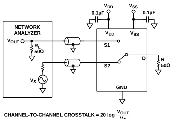
Figure 29. Channel-to-Channel Crosstalk
