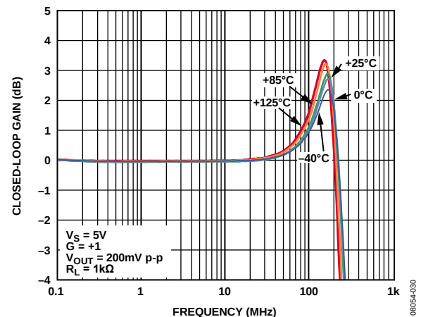
Figure 9. Small-Signal Frequency Response vs. Temperature, V_S = 5\text{ V} , ADA4891-1/ADA4891-2
