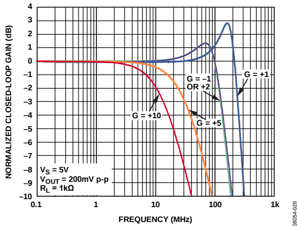
Figure 7. Small-Signal Frequency Response vs. Gain, V_S = 5\text{ V} , ADA4891-1/ADA4891-2
