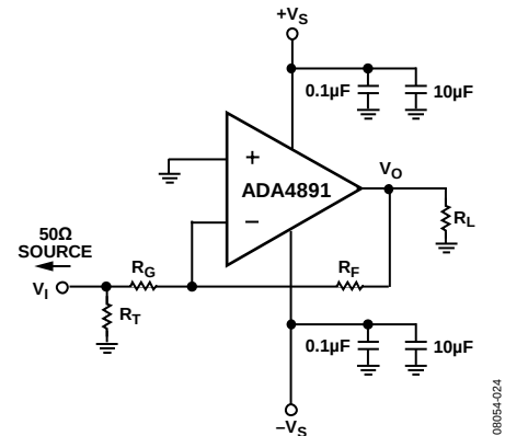
Figure 51. Inverting Gain Configuration
