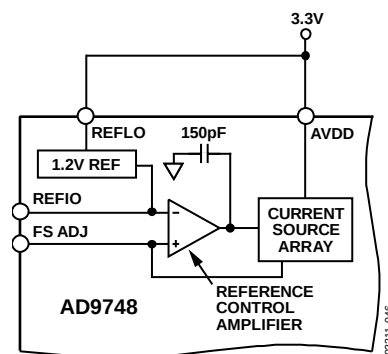
Figure 18. External Reference Configuration
