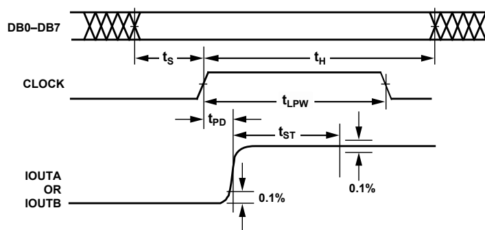
Figure 2. Timing Diagram
