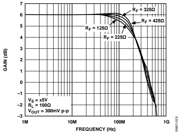
Figure 29. AD9632 Small Signal Frequency Response, G = +2
