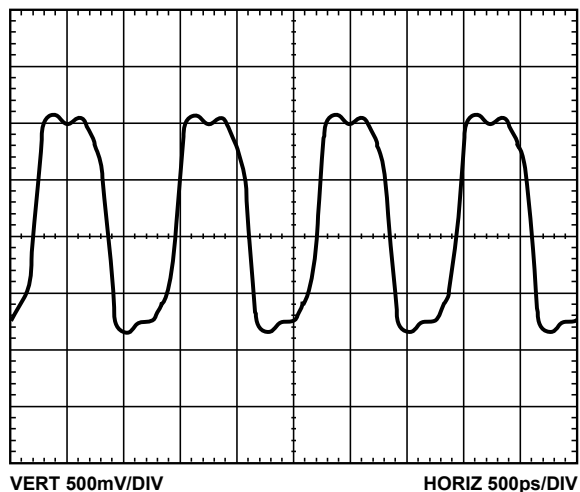
Figure 18. LVPECL Differential Output @ 800 MHz
