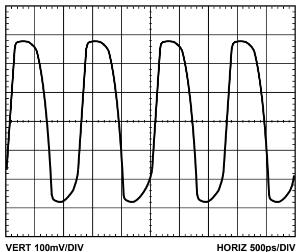
Figure 19. LVDS Differential Output @ 800 MHz
