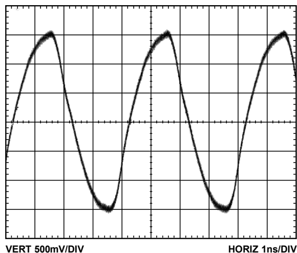
Figure 20. CMOS Single-Ended Output @ 250 MHz with 10 pF Load
