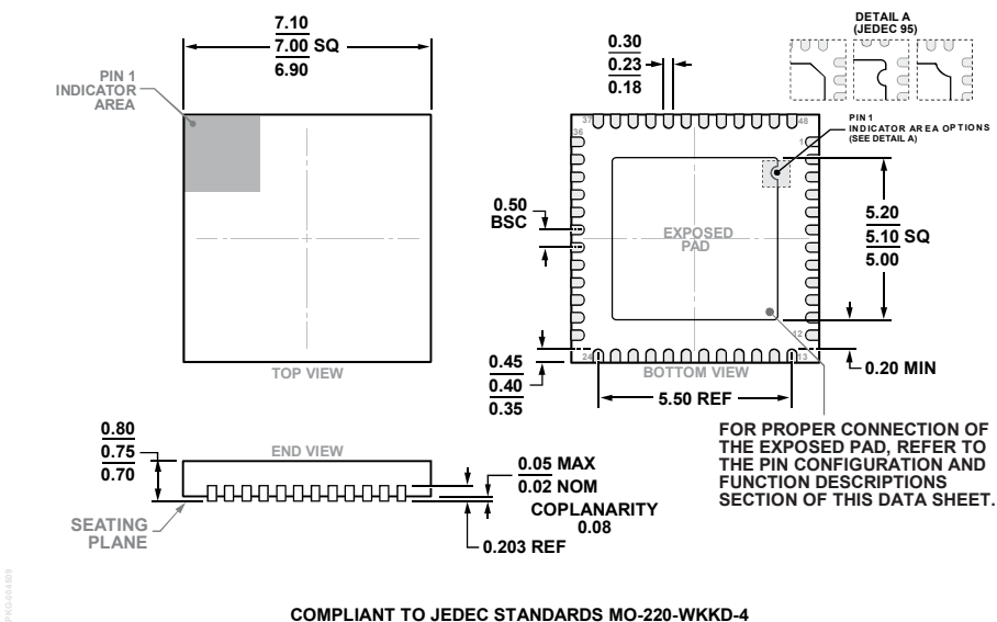
Figure 45. 48-Lead Lead Frame Chip Scale Package [LFCSP] 7 mm × 7 mm Body and 0.75 mm Package Height (CP-48-4) Dimensions shown in millimeters
