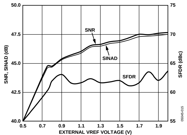
Figure 15. SNR, SINAD, and SFDR vs. V_{REF} in External Reference Mode, A_{IN} = 70 \text{ MHz} @ -1 \text{ dBFS}, 250 \text{ MSPS}
