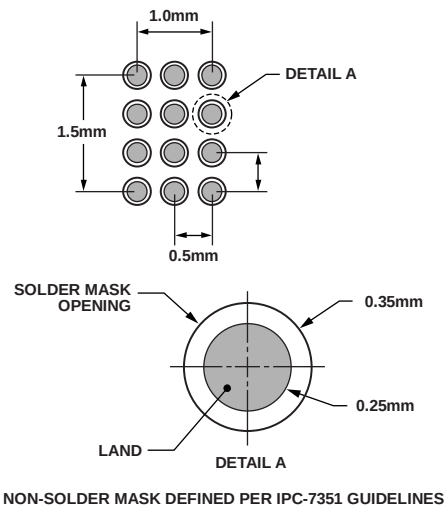
Figure 6. Recommended Solder Land Pattern
