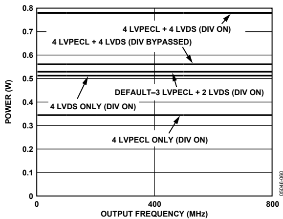
Figure 7. Power vs. Frequency—LVPECL, LVDS (PLL Off)
