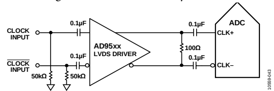
Figure 47. Differential LVDS Sample Clock (Up to 625 MHz)
