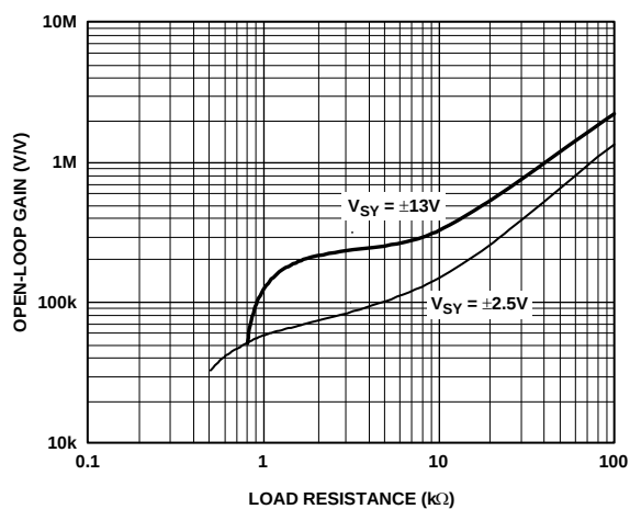
Figure 17. Open-Loop Gain vs. Load Resistance
