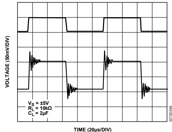
Figure 48. AD8610/AD8620 Capacitive Load Drive, A_V = +2
