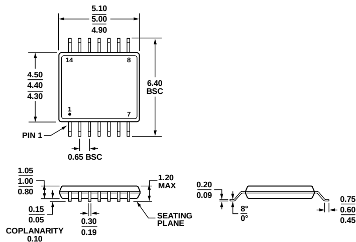
Figure 66. 14-Lead Thin Shrink Small Outline Package [TSSOP] (RU-14) Dimensions shown in millimeters
