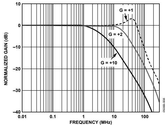
Figure 11. Small Signal Frequency Response for Various Gains ( V_S = \pm 5\text{ V} , V_O = 0.1\text{ V p-p} , R_L = 25\ \Omega )
