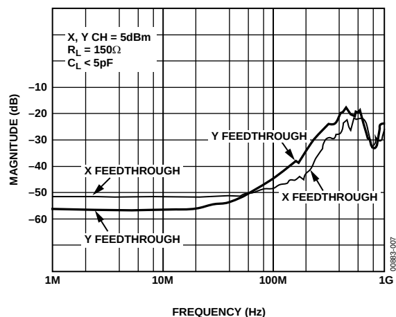
Figure 7. X and Y Feedthrough vs. Frequency
