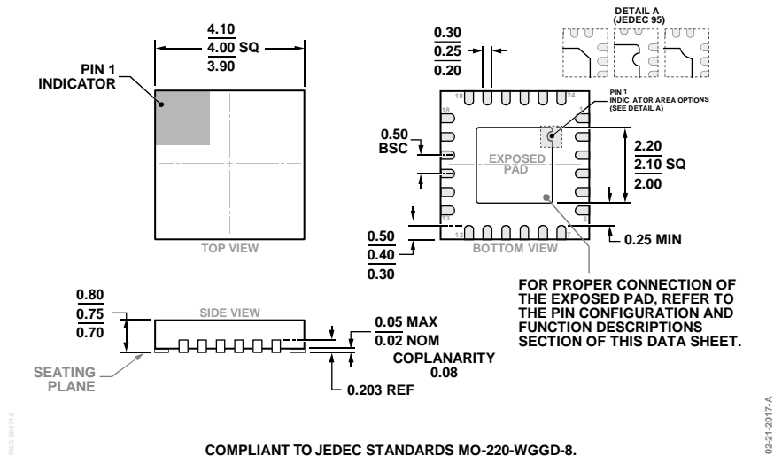
COMPLIANT TO JEDEC STANDARDS MO-220-WGGD-8. Figure 44. 24-Lead Lead Frame Chip Scale Package [LFCSP] 4 mm × 4 mm Body and 0.75 mm Package Height (CP-24-10) Dimensions shown in millimeters
