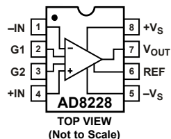
Figure 44. Pinout Diagram
