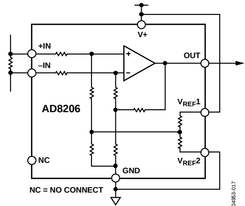
Figure 20. Split Supply
