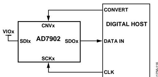
Figure 38. \overline{\text{CS}} Mode, 3-Wire Interface Without a Busy Indicator Connection Diagram ( \text{SDIx} High)
