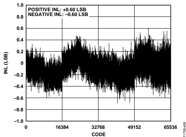
Figure 6. Integral Nonlinearity vs. Code, V_{REF} = 2.5\text{ V}
