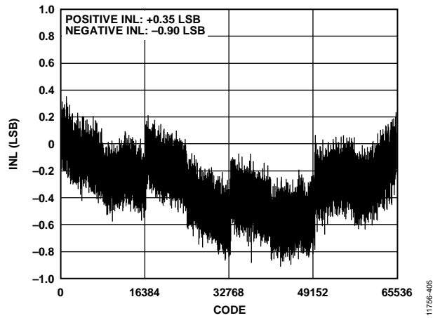
Figure 5. Integral Nonlinearity vs. Code, V_{REF} = 5\text{ V}
