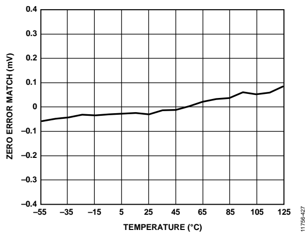
Figure 27. Zero Error Match vs. Temperature
