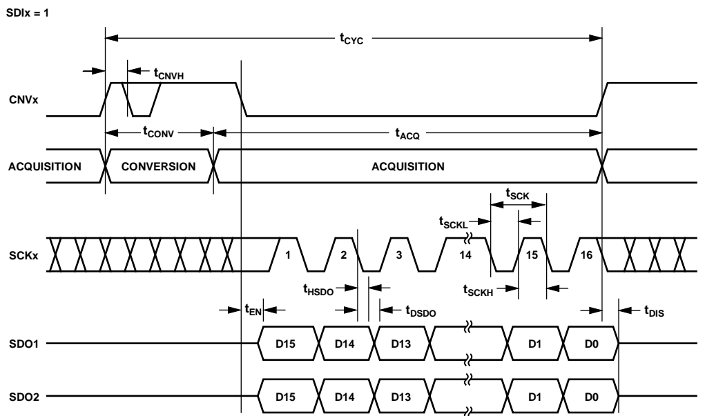
Figure 51. Potential Simultaneous Sampling Serial Interface Timing
