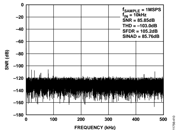
Figure 10. FFT Plot, V_{REF} = 2.5\text{ V}
