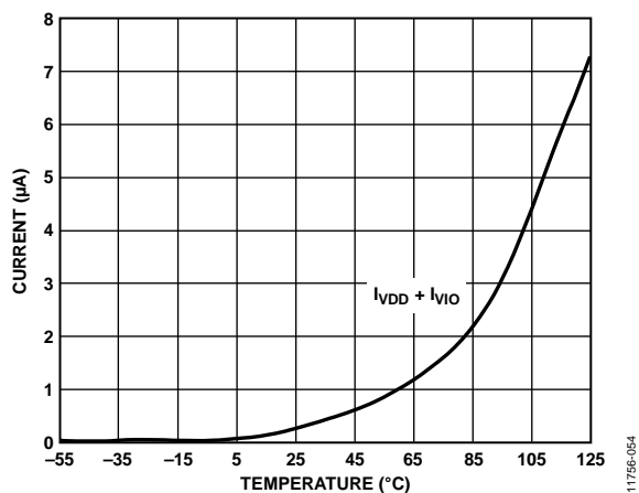
Figure 26. Power-Down Current for Each ADC vs. Temperature
