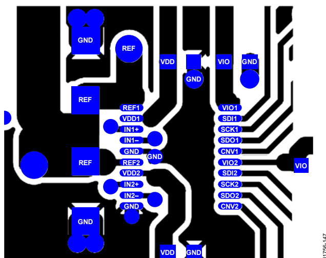
Figure 53. Example Layout of the AD7902 (Top Layer)
