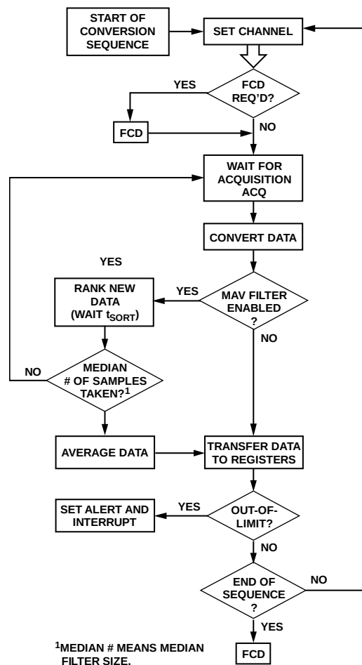
Figure 34. Conversion Sequence
