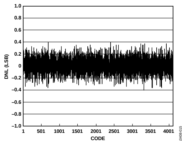
Figure 15. ADC DNL
