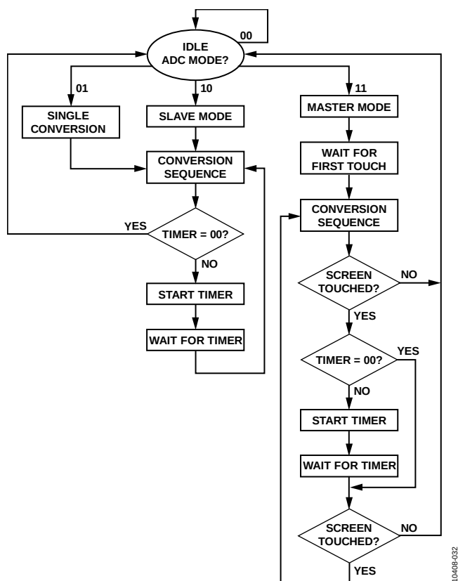
Figure 33. Conversion Modes
