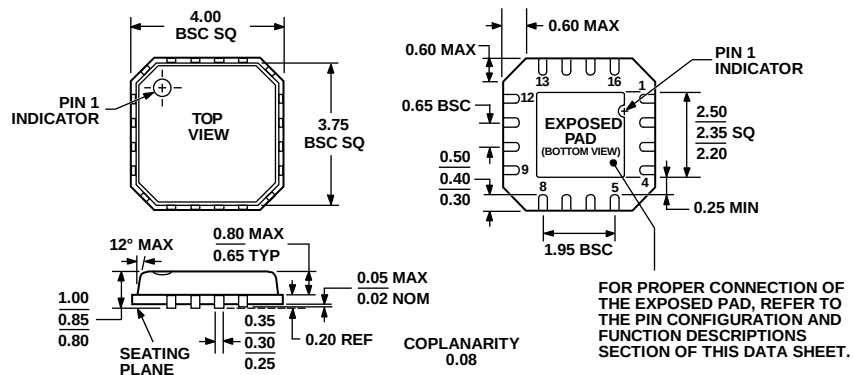
Figure 48. 16-Lead Lead Frame Chip Scale Package [LFCSP_VQ] 4 mm × 4 mm, Very Thin Quad (CP-16-10)
