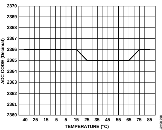
Figure 18. ADC Code vs. Temperature (Fixed Analog Input)
