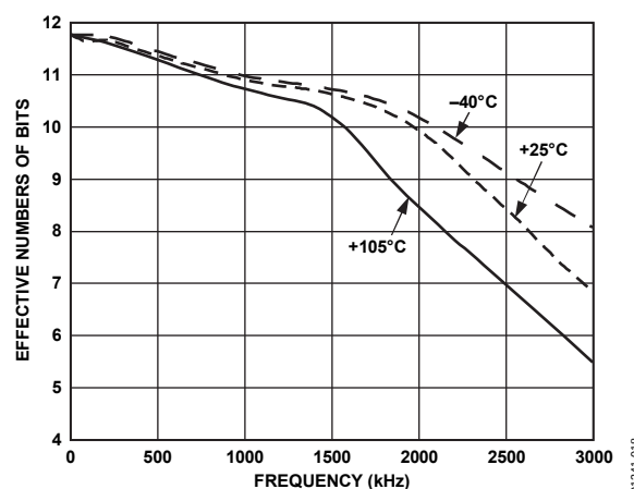
Figure 18. Effective Numbers of Bits vs. Frequency
