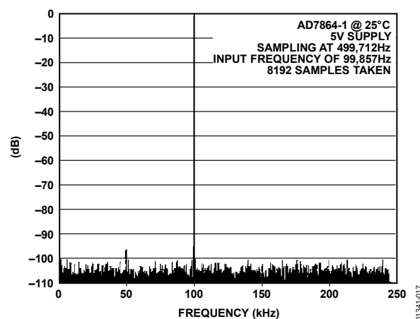
Figure 17. FFT Plot
