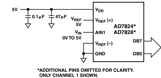
Figure 10. AD7824/AD7828 Unipolar 0 V to 5 V Operation
