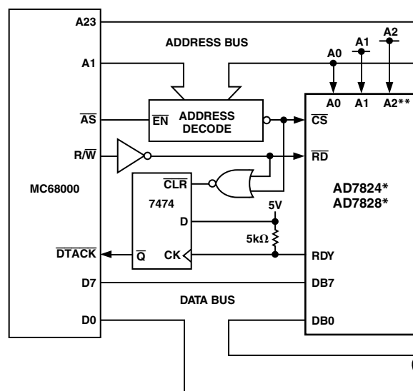
Figure 17. AD7824/AD7828–MC68000 Interface
