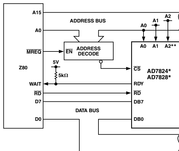
Figure 16. AD7824/AD7828–Z80 Interface
