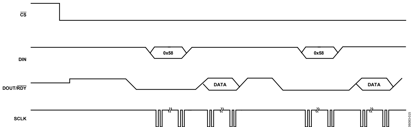
Figure 15. Continuous Conversion
