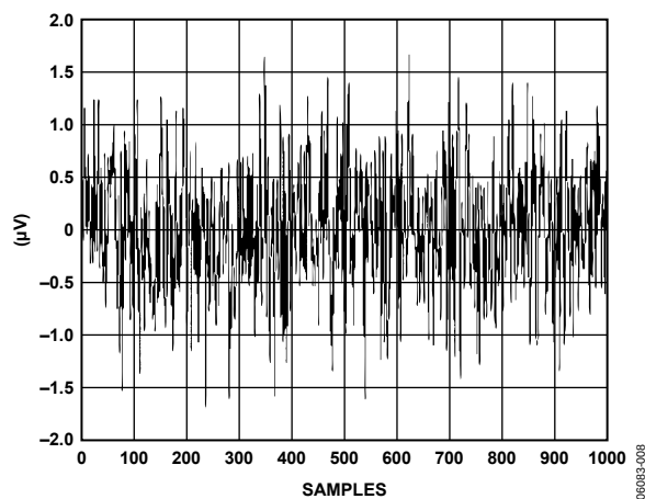
Figure 8. AD7797 Noise ( V_{REF} = AV_{DD} , Update Rate = 4.17 Hz)
