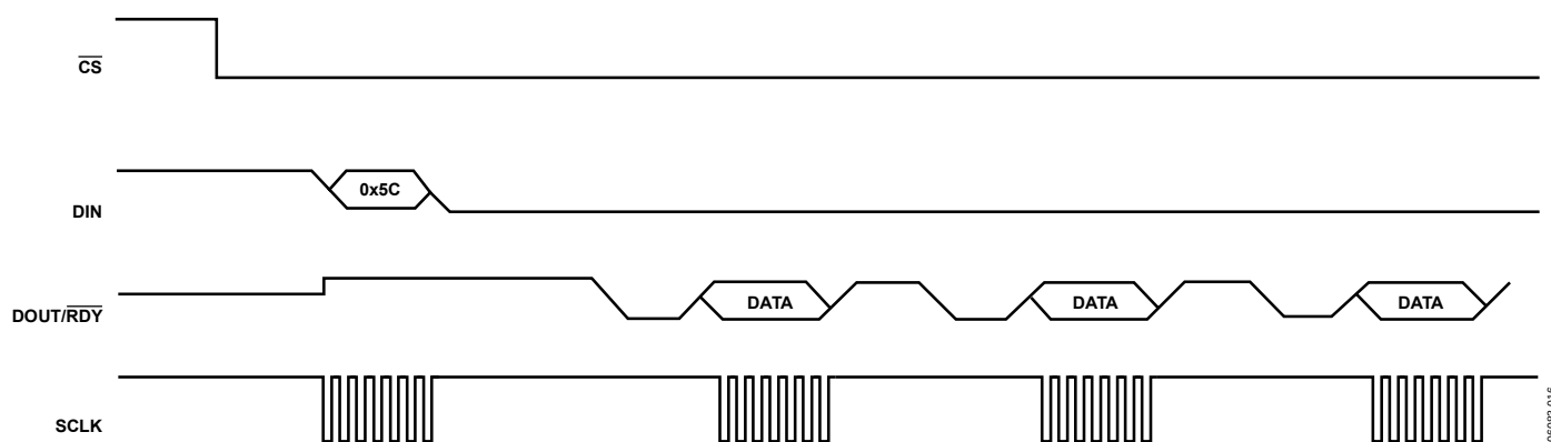
Figure 16. Continuous Read
