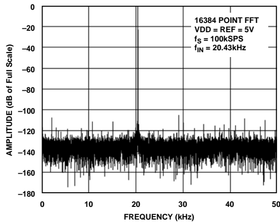
Figure 9. FFT Plot
