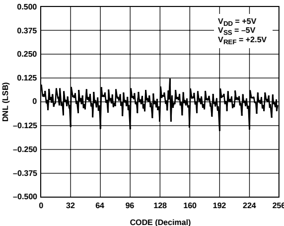
Figure 14. DNL vs. Code
