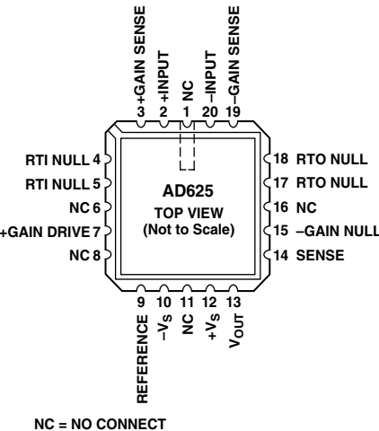
Leadless Chip Carrier (E) Package
