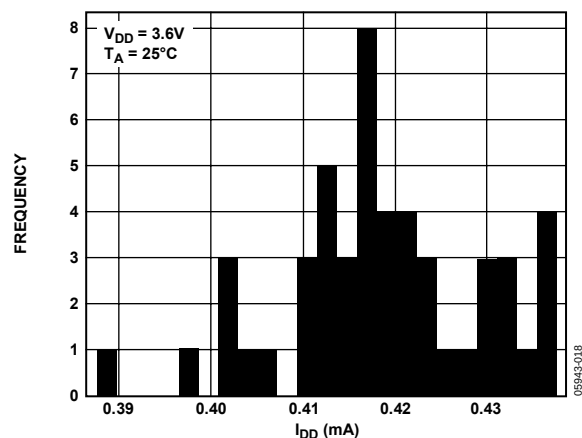
Figure 16. I_{DD} Histogram with V_{DD} = 3.6\text{ V}
