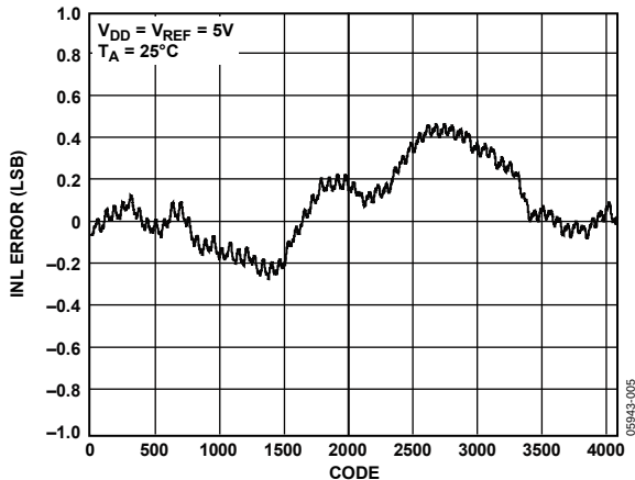
Figure 5. INL AD5624
