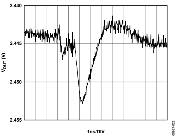
Figure 23. Digital Feedthrough
