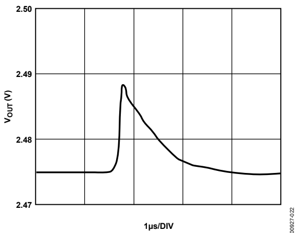
Figure 22. Major-Code Transition
