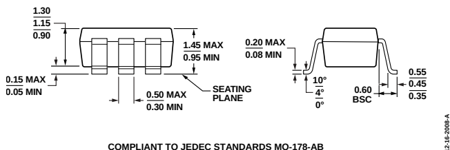
Figure 35. 6-Lead Small Outline Transistor Package [SOT-23] (RJ-6)
