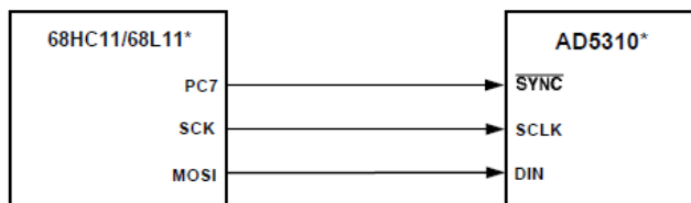
Figure 29. AD5310 to 68HC11/68L11 Interface
