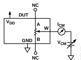
Figure 32. Common-Mode Leakage Current
