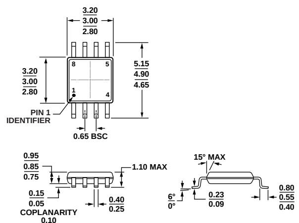
COMPLIANT TO JEDEC STANDARDS MO-187-AA Figure 41. 8-Lead Mini Small Outline Package [MSOP] (RM-8)
