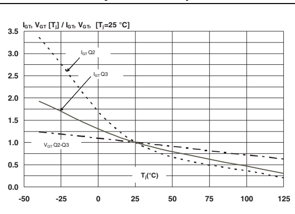
Figure 7. Relative variation of I_{GT} and V_{GT} versus junction temperature
