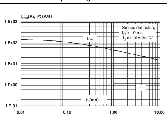
Figure 9. Non repetitive surge peak on-state current for a sinusoidal pulse, and corresponding value of I^2t
