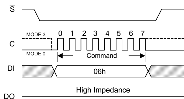
Figure 15-1. Write Enable (WREN) Sequence (Command 06) (SPI Mode)
