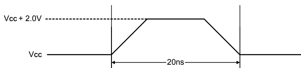
Figure 10. Maximum Positive Input Overshoot
