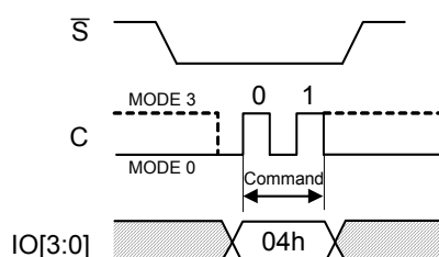
Figure 16-2. Write Disable (WRDI) Sequence (Command 04) (QPI Mode)
