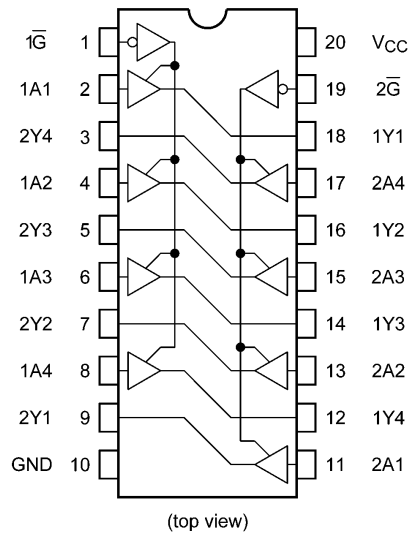
74VHCT244AFT
