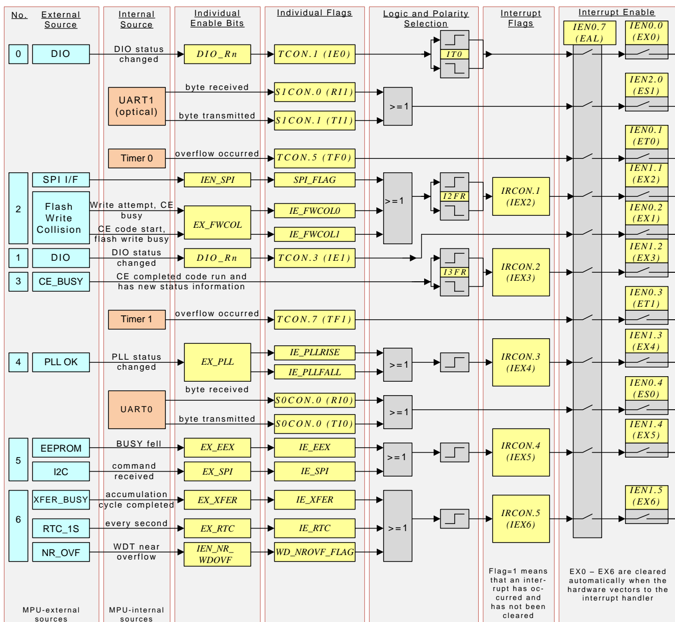
Figure 7: Interrupt Structure
