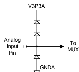
Analog Input Equivalent Circuit
