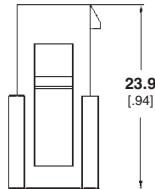
Recommended Cutout for 2.00 [.079] Max. Thick Panel
