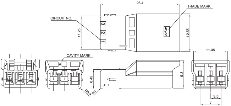
Cap Housing (For Tabs)
