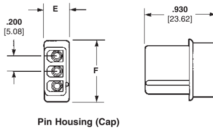
Pin Housing (Cap)
