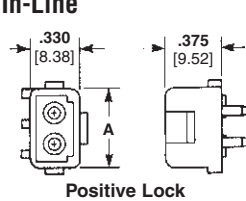
Positive Lock
