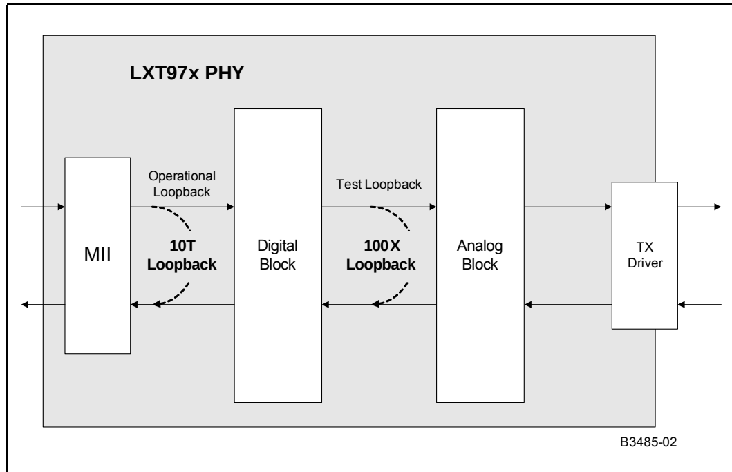
Figure 10 Loopback Paths
