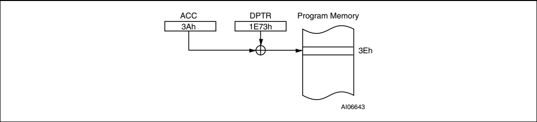
Figure 12. Indexed addressing
