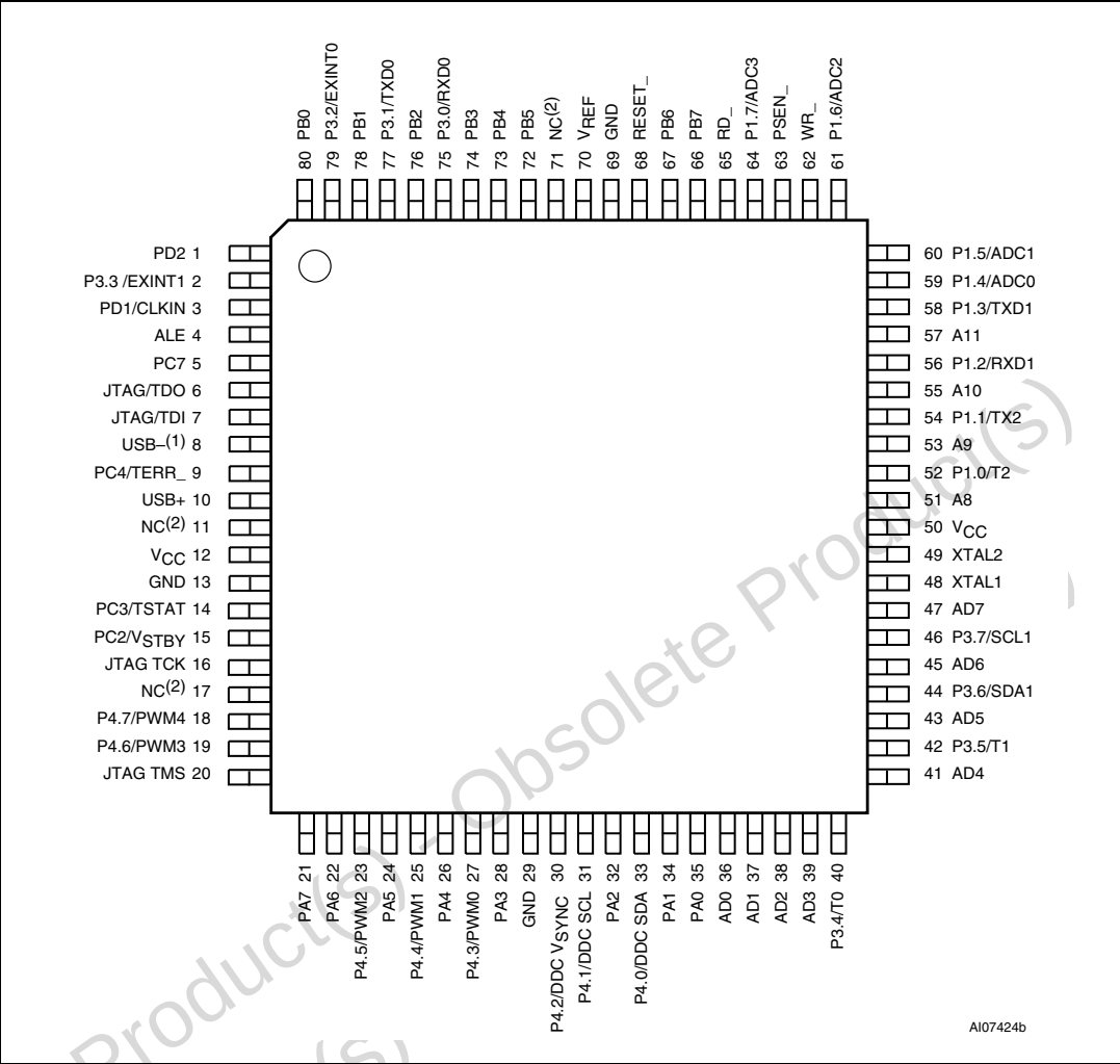
Figure 3. TQFP80 connections
