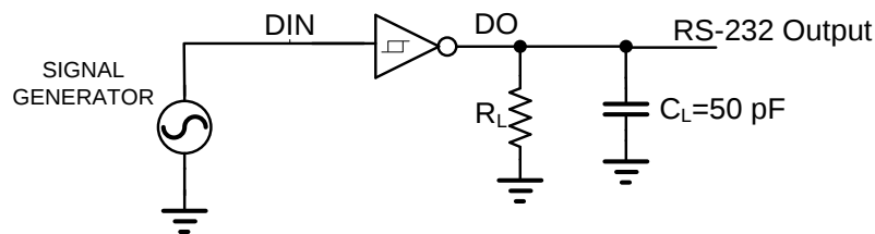
Test Circuit
