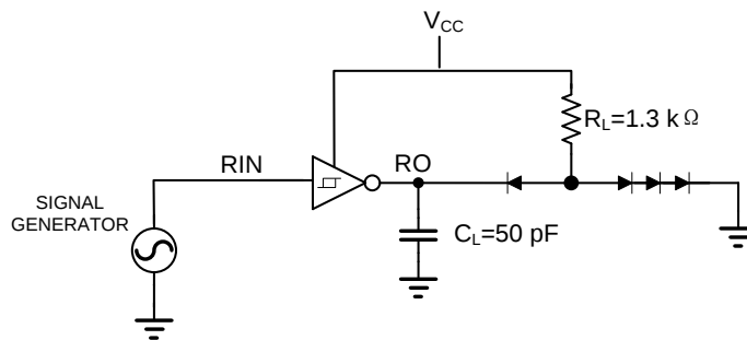
Test Circuit
