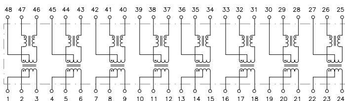
Circuit A
