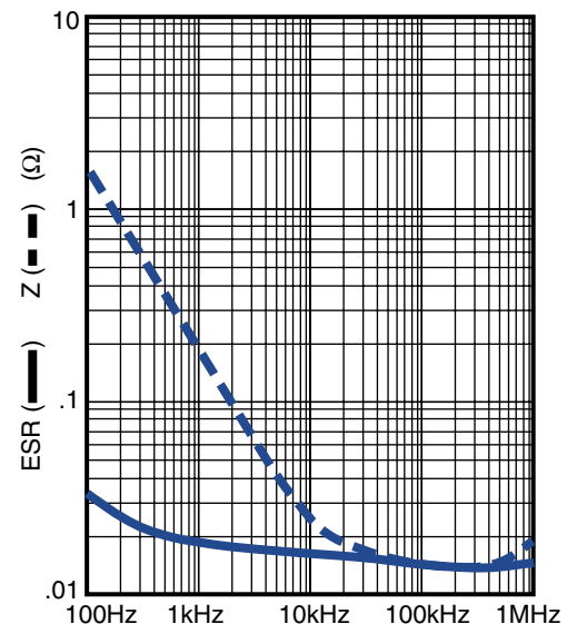
TYPICAL ESR/Z FREQUENCY SCAN @ 25°C
