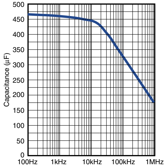
TYPICAL CAP FREQUENCY SCAN @ 25°C
