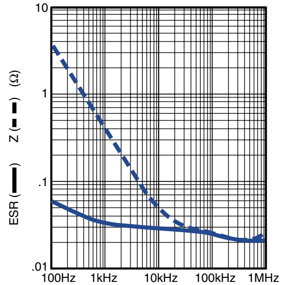
TYPICAL ESR/Z FREQUENCY SCAN @ 25°C
