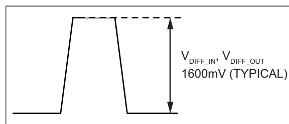
FIGURE 4-2: Differential Swing.
