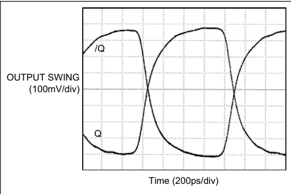
FIGURE 2-3: 622 MHz Output.
