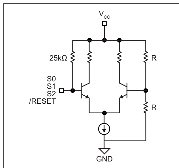
FIGURE 4-4: Differential Input Structure.
