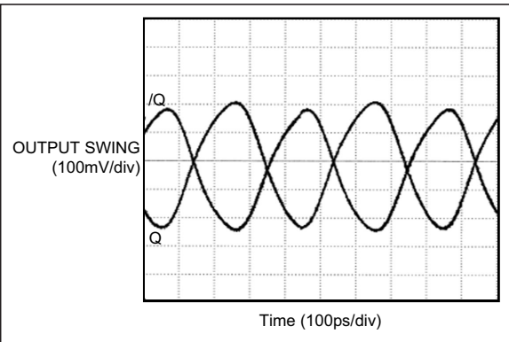
FIGURE 2-5: 2.5 GHz Output.
