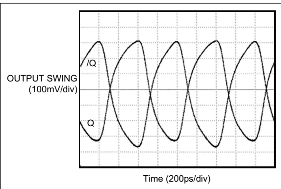
FIGURE 2-4: 1.25 GHz Output.
