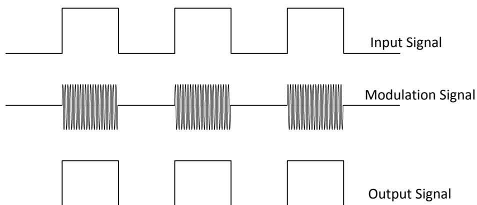
Figure 3.5. Modulation Scheme
