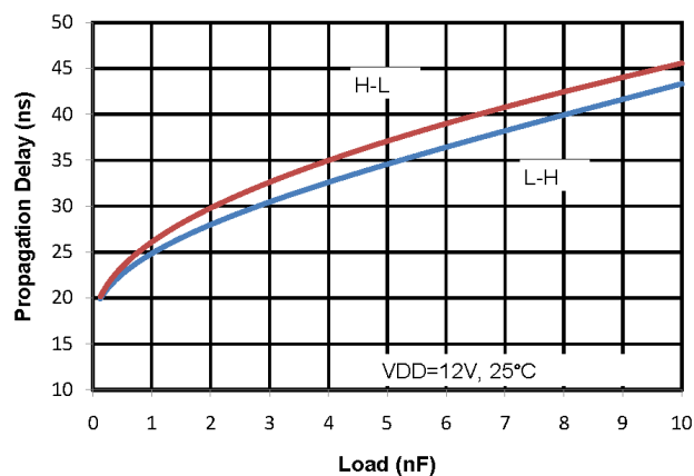
Figure 3.21. Propagation Delay vs. Load
