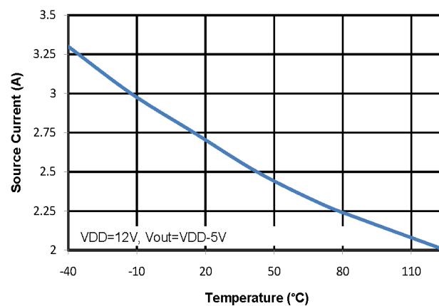
Figure 3.27. Output Source Current vs. Temperature
