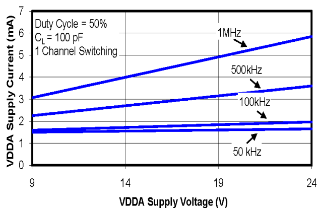
Figure 3.12. Supply Current vs. Supply Voltage
