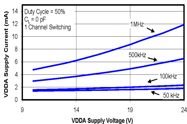
Figure 3.25. Supply Current vs. Supply Voltage
