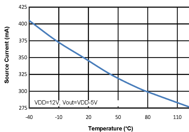
Figure 3.15. Output Source Current vs. Temperature
