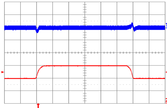
Fig. 9: Output voltage response to load current step-change (20 A 30 A – 20 A) at V_{in} = 48\text{ V} . Top trace: output voltage (100 mV/div.). Bottom trace: load current (10 A/div.). Current slew rate: 0.1 A/ \mu\text{s} C_o = 1\text{ }\mu\text{F} ceramic. Time scale: 0.2 ms/div
