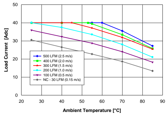
Fig. 2: Available load current vs. ambient air temperature and airflow rates for converter with G height pins mounted horizontally with air flowing from pin 1 to pin 3, MOSFET temperature \leq 120^\circ\text{C} , V_{in} = 48\text{ V}
