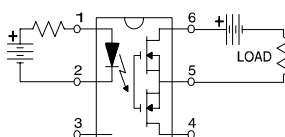
"B" Connection
