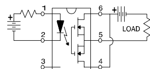
"C" Connection
