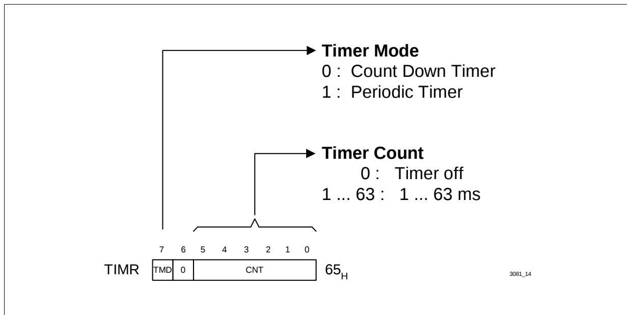
Figure 11 Timer Register
