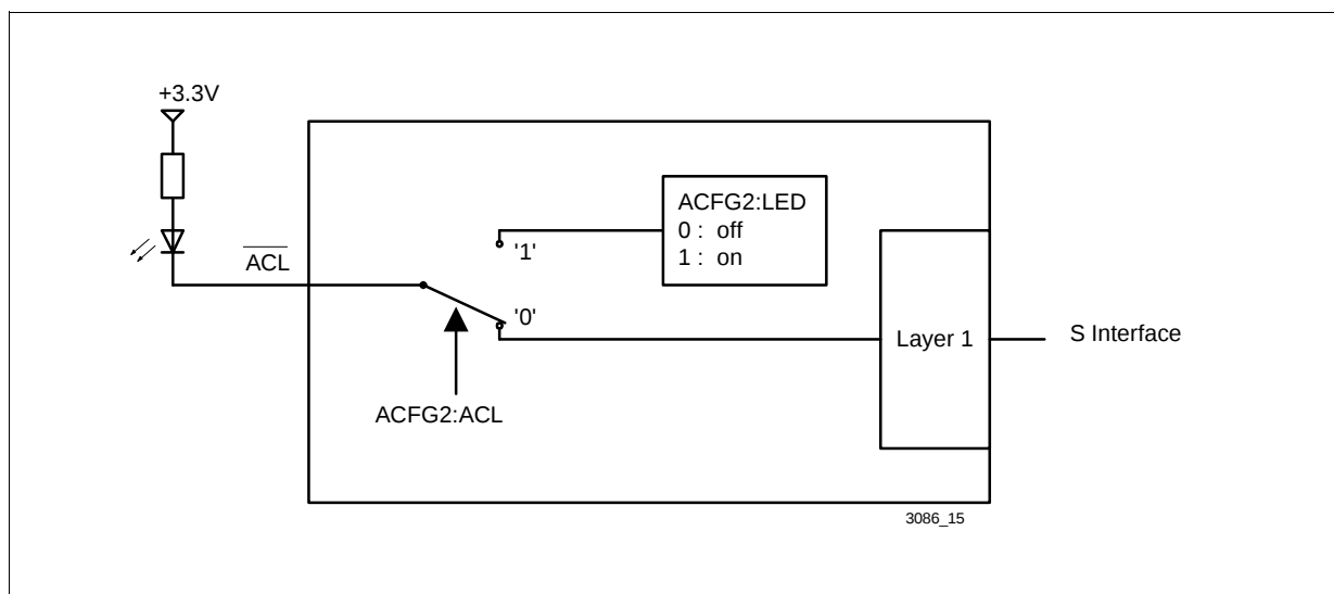
Figure 13 ACL Configuration
