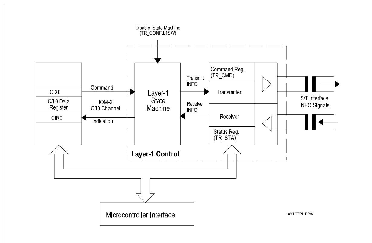
Figure 31 Layer-1 Control
