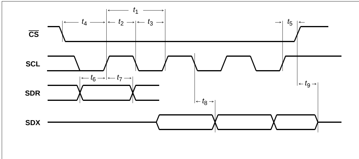
Figure 72 SCI Interface
