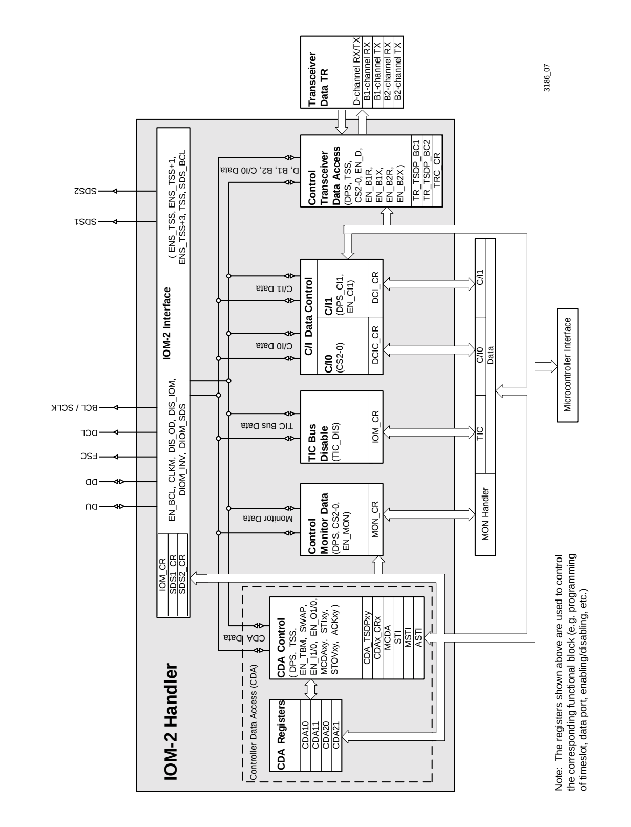
Figure 42 Architecture of the IOM Handler (Example Configuration)
